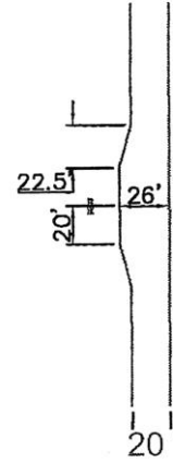
MINIMUM CLEARANCE AROUND A FIRE HYDRANT
