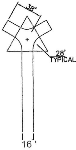
ACCEPTABLE ALTERNATIVE TO 72' HAMMERHEAD Private
