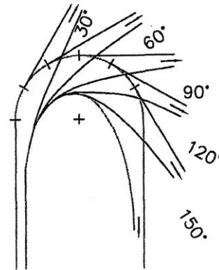
STAA TRUCK SEMITRAILER WHEEL TRACKS 50' TURNING RADIUS
