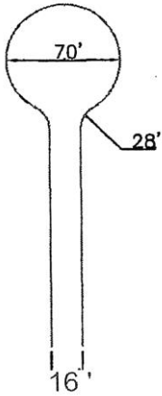
70' DIAMETER CUL-DE-SAC Private
