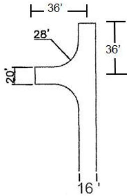
ACCEPTABLE ALTERNATIVE TO 72' HAMMERHEAD Private
